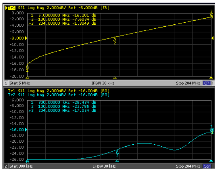
SRE-M-16
